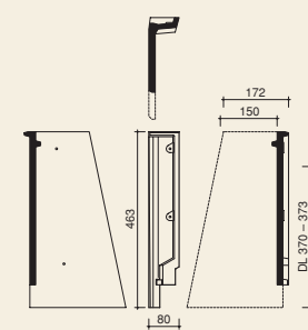
Ortgangsteg, links
